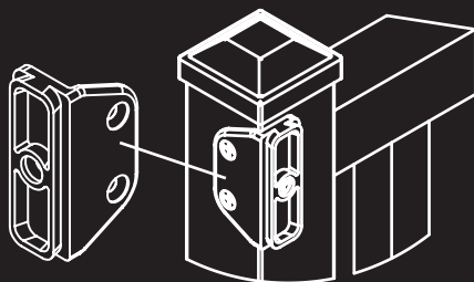
Top Bracket
